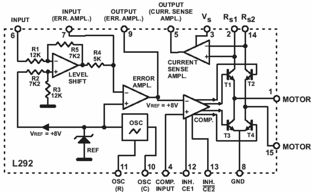
Fig. 1. The block diagram of the L292 integrated circuit.
