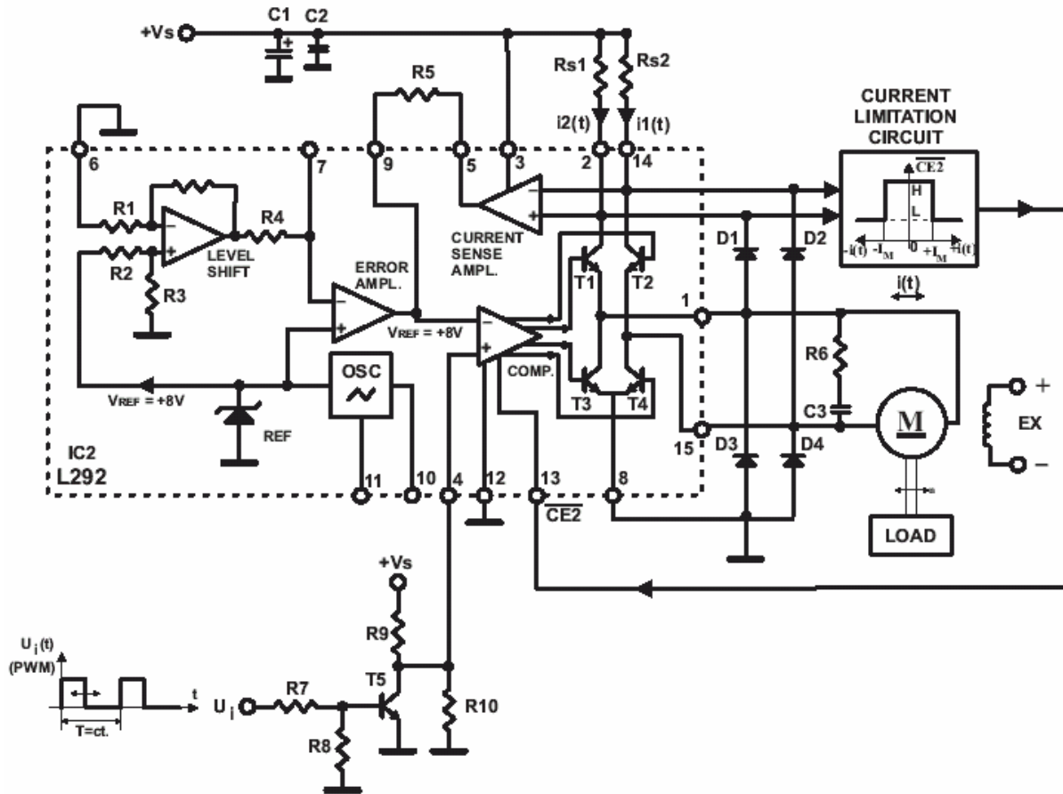
Fig. 2. The electrical block diagram of the realized system.
