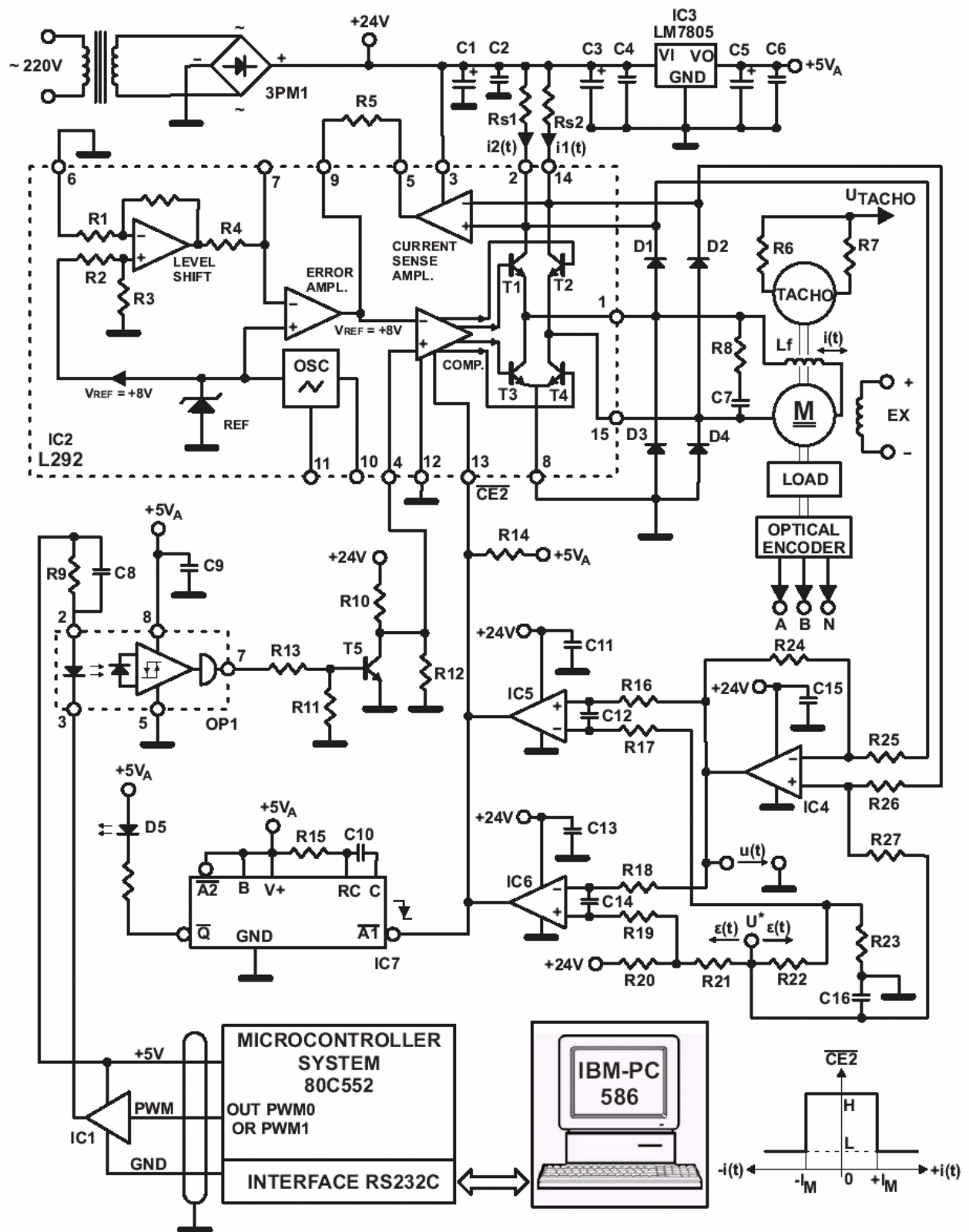
Fig. 3. The electrical schematic of realized system.
